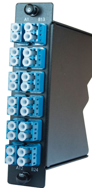
24 Fiber LC to Dual 12 Fiber MPO
