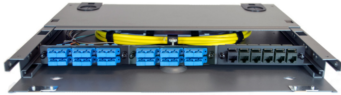
1RU RDR Rackmount Panel with CAT 6 Keystone Jacks
